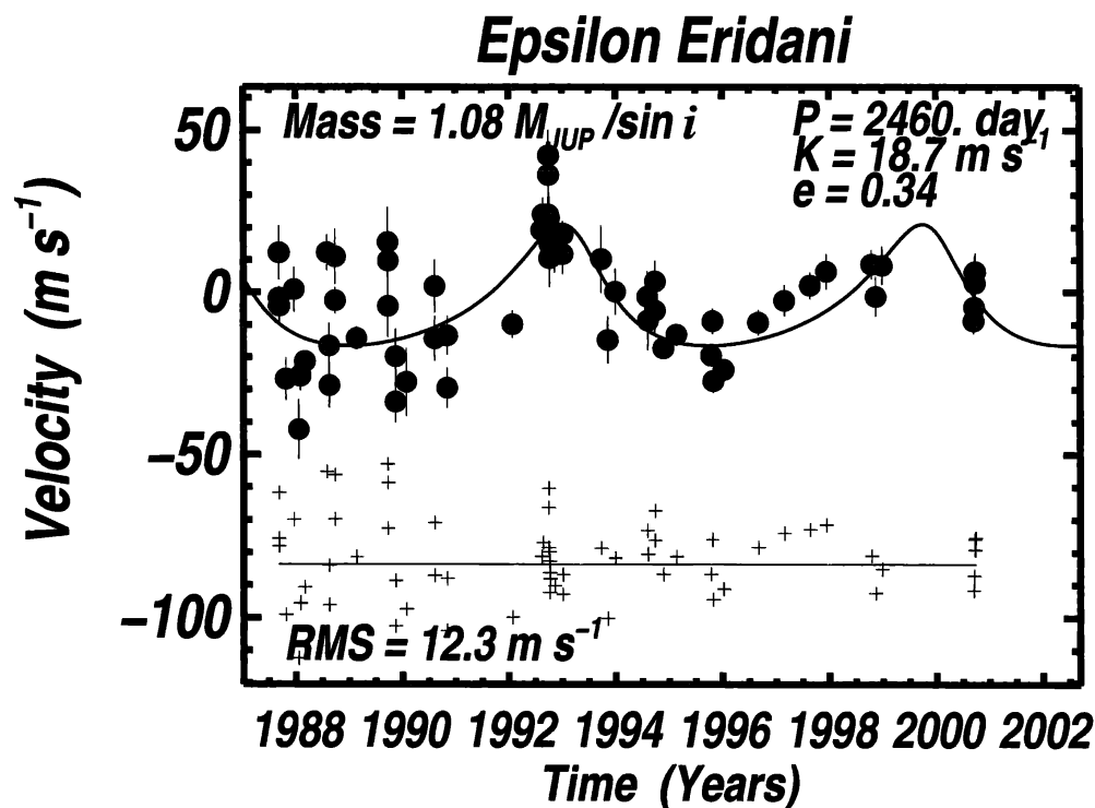
Figure 2. Doppler jitter of 15\text{--}20\text{ m s}^{-1} , caused by magnetic activity in FGK stars younger than 1 Gyr. The 1 Gyr-old star, \epsilon Eri, exhibits jitter of 15\text{ m s}^{-1} . Subtraction of a possible orbit (solid line) leaves residuals (crosses) that have RMS of 12.3\text{ m s}^{-1} , far greater than errors (see error bars). The credibility of the Keplerian variation is weakened by Doppler jitter, as is the detectability of additional planets.
